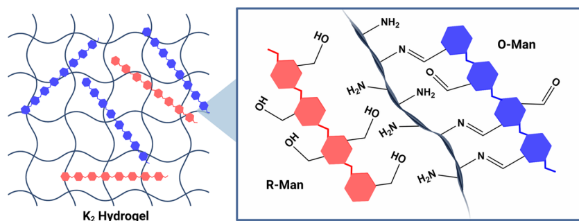
Figure 1. Schematic showing O-Man (blue) and R-Man (red) loaded into a K_2 hydrogel. Aldehyde groups on O-Man can form imine bonds with the amines on the K_2 peptide fibers whereas the hydroxyl groups present on R-Man cannot form imine bonds with K_2 .
