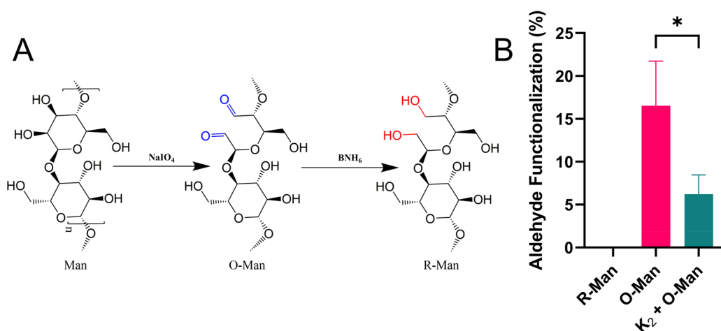
Figure 2. (A) Schematic of oxidation and reduction reactions on a representative portion of the linear mannan polysaccharide showing one mannose monomer being oxidized and then subsequently reduced. (B) Results of the fluorometric aldehyde quantification assay show the percent of mannose monomers oxidized, referred to as aldehyde functionalization, for O-Man and R-Man. Mixing O-Man with K 2 led to a significant decrease in aldehyde content, suggesting the formation of imine bonds between the peptide and the carbohydrate.
